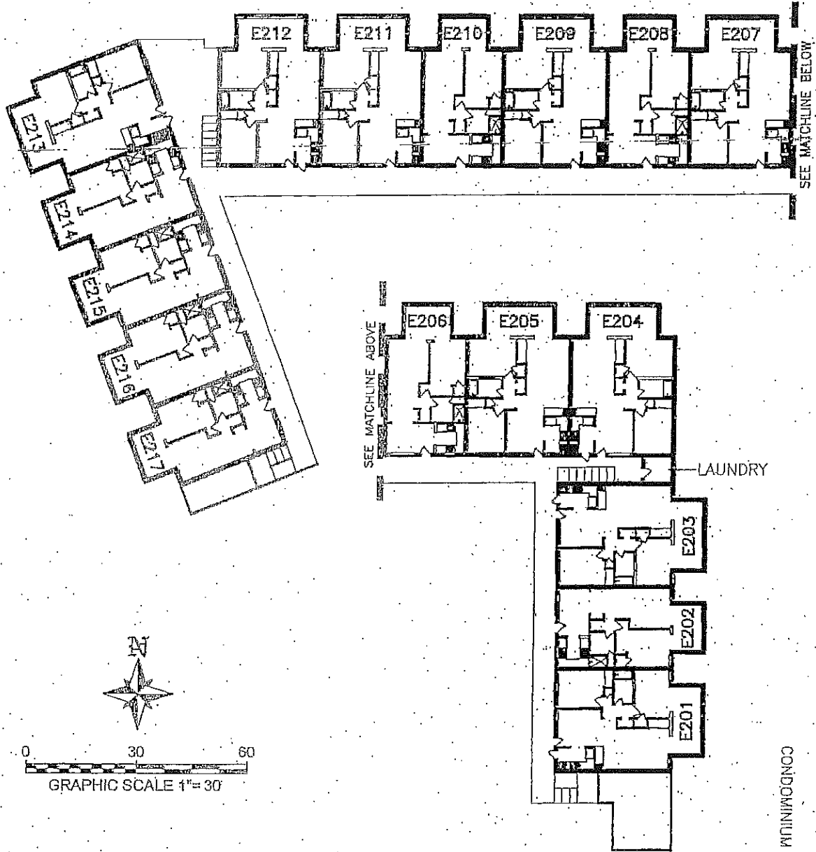
BUILDING "E" SECOND FLOOR PLAN EXHIBIT "A"
