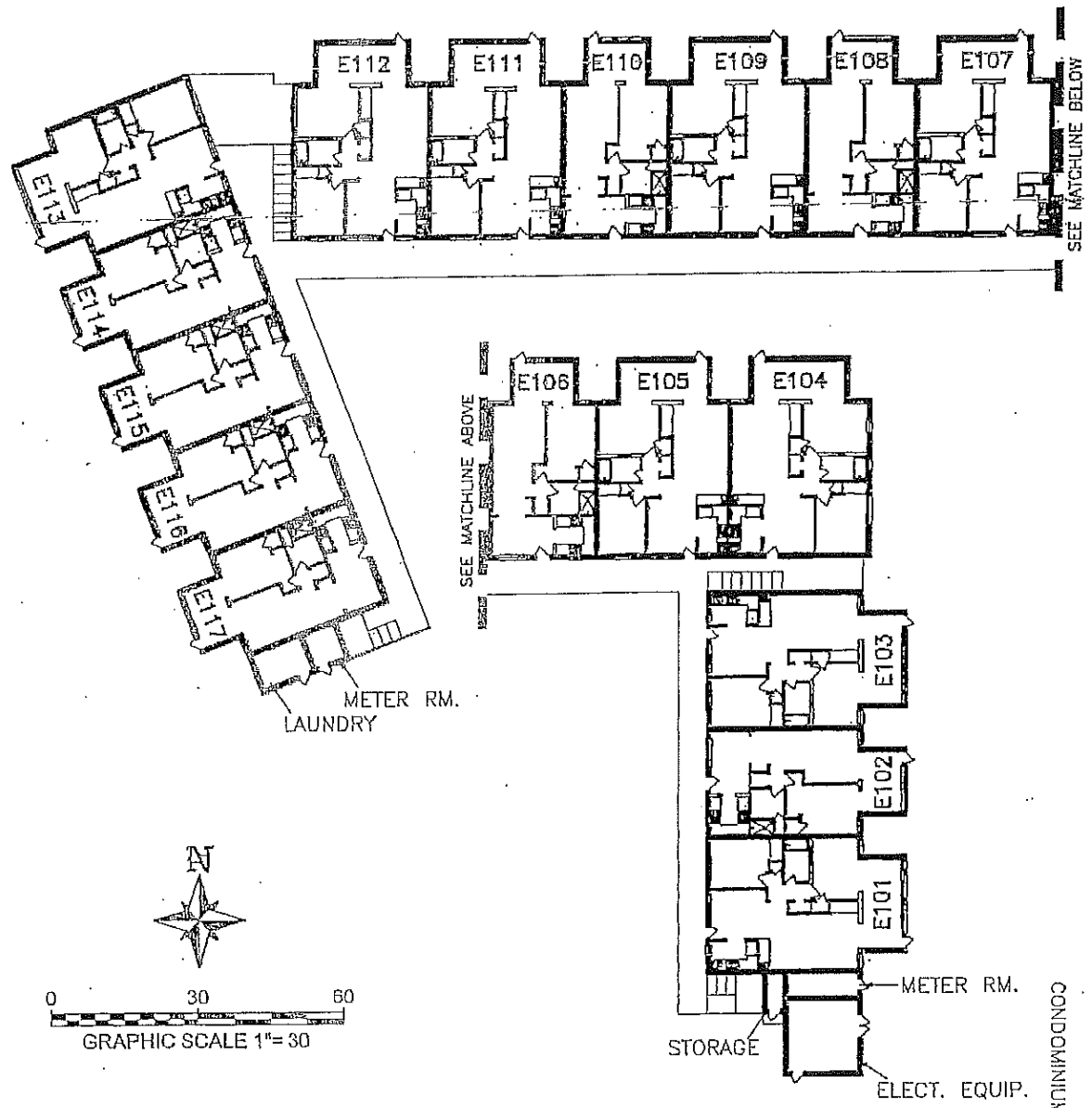
BUILDING "E" FIRST FLOOR PLAN EXHIBIT "A"
